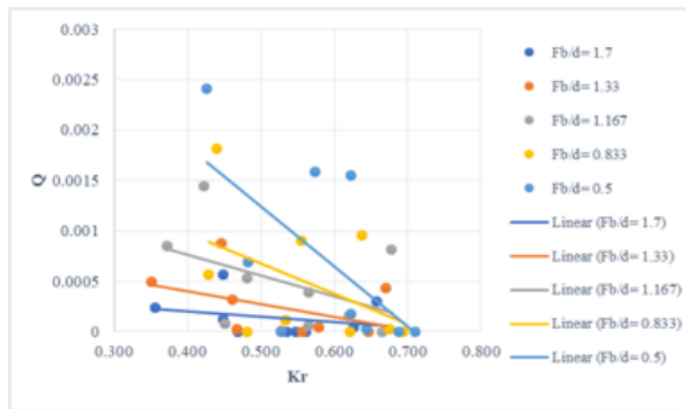
Figure 9. Graph of the relationship of K_r to Q at d = 0.3 m Source: (Results of data processing, 2021)
