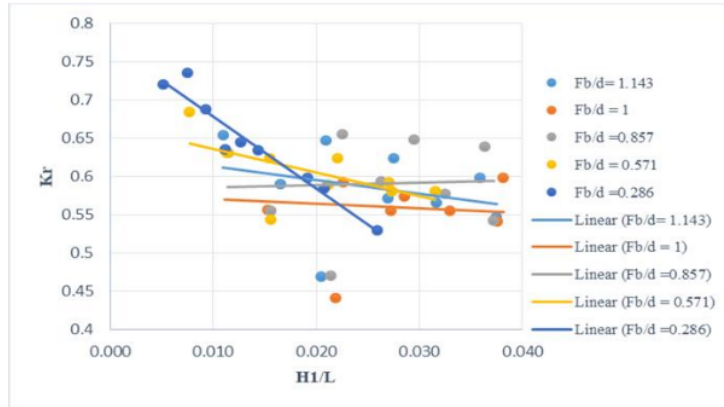
Figure 7. Graph of the relationship between H1/L and Kr at d=0.35 m Source: (Results of data processing, 2021)
