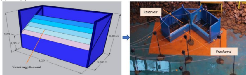
Figure 2. Model and model dimensions (Source: Lab LK, 2021)
